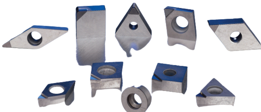
PCD/PCBN TURNING INSERT
